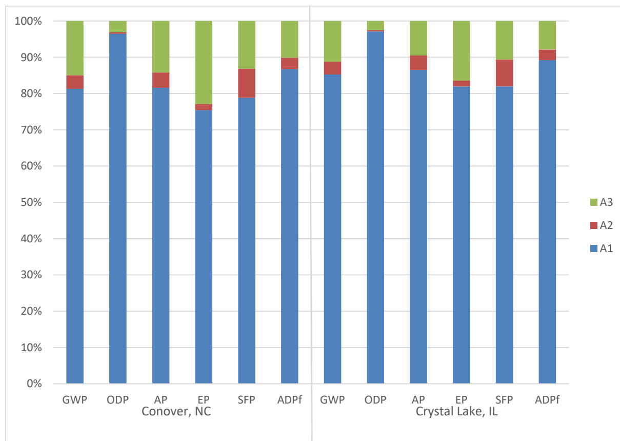
Figure 3. Contribution analysis of the Camfil Hi-Flo ES MERV 13 filter.
